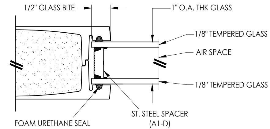
G1 GLAZING DETAIL CLEAR GLASS
