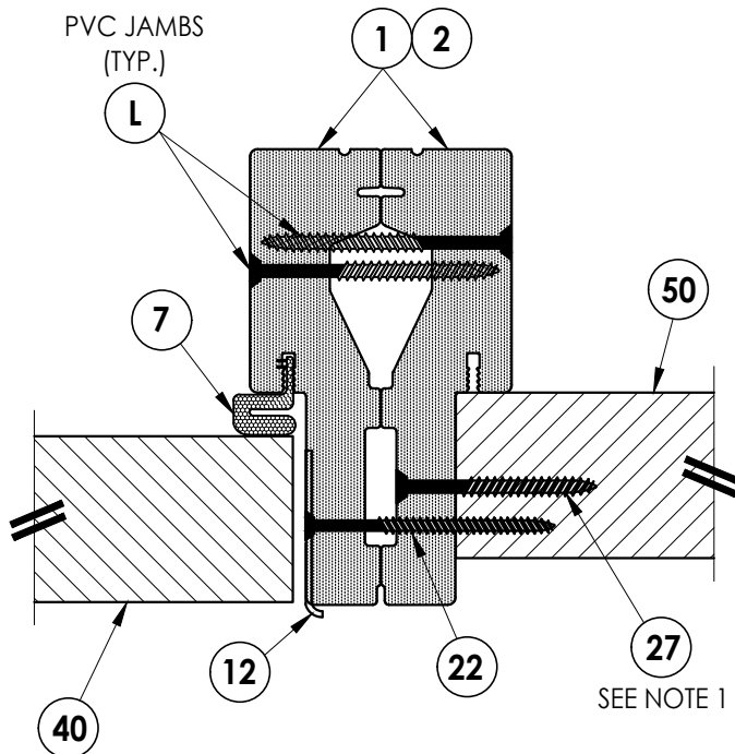
2 5 HORIZONTAL CROSS SECTION
