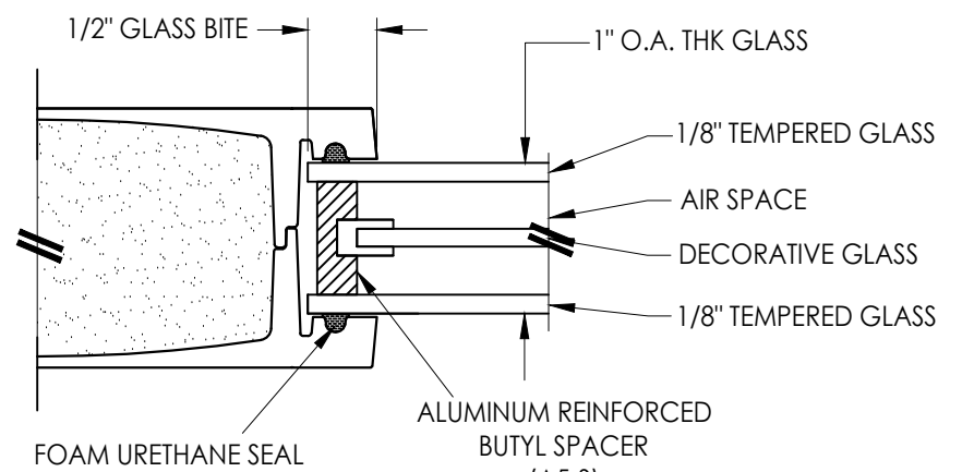
G2 GLAZING DETAIL DECORATIVE GLASS
